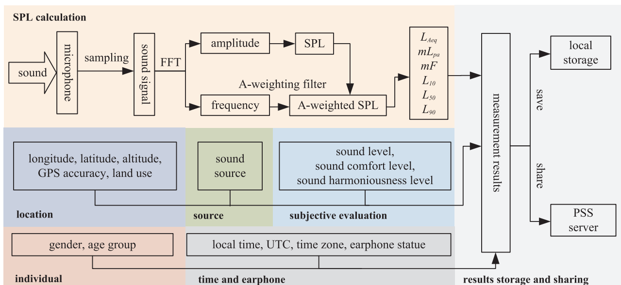
Fig. 1. Logical architecture for SPL Meter.
